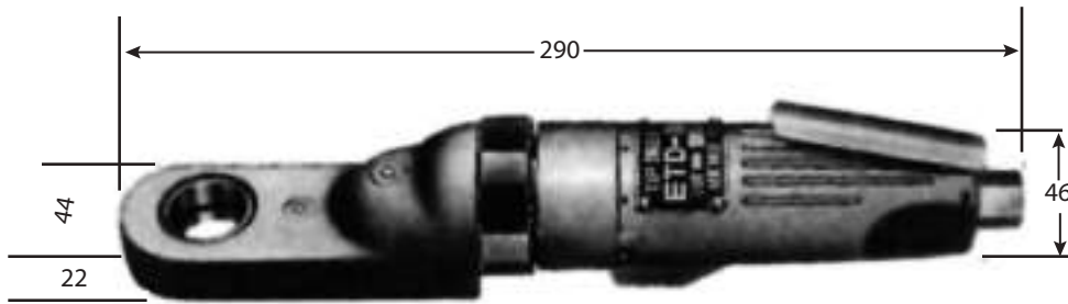
Tip Dresser
